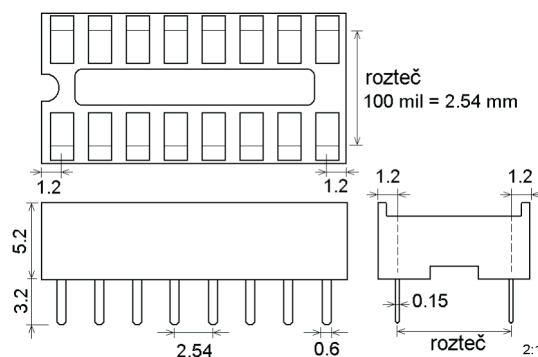
DIL - 28 / 3 YT - 1
