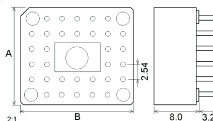
PLCC - 32 T - 1
