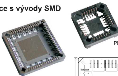
PLCC - 68 NTT - 5 SMD
