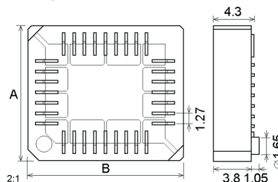
PLCC - 44 NTT - 5 SMD
